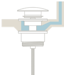
SLOTTED (Use with basin with overflow)
